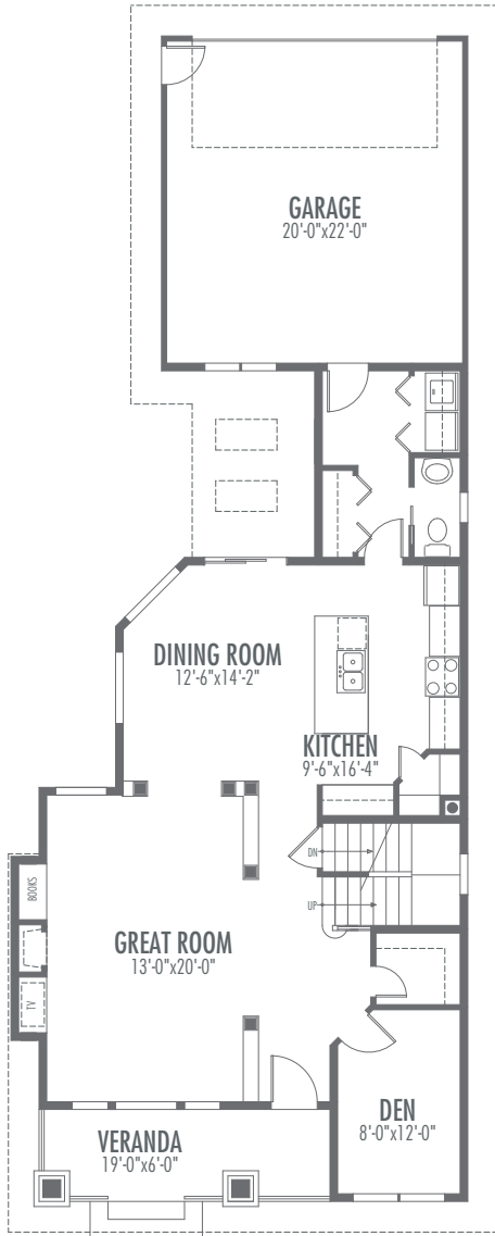
MAIN FLOOR AREA: 1125 SQ. FT.
