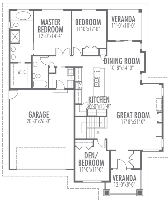
MAIN FLOOR AREA: 1782 SQ. FT.
