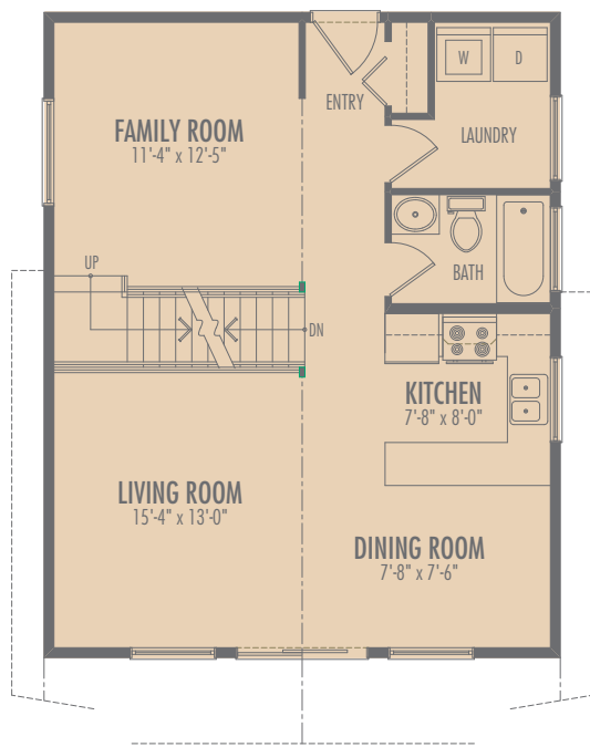
MAIN FLOOR
