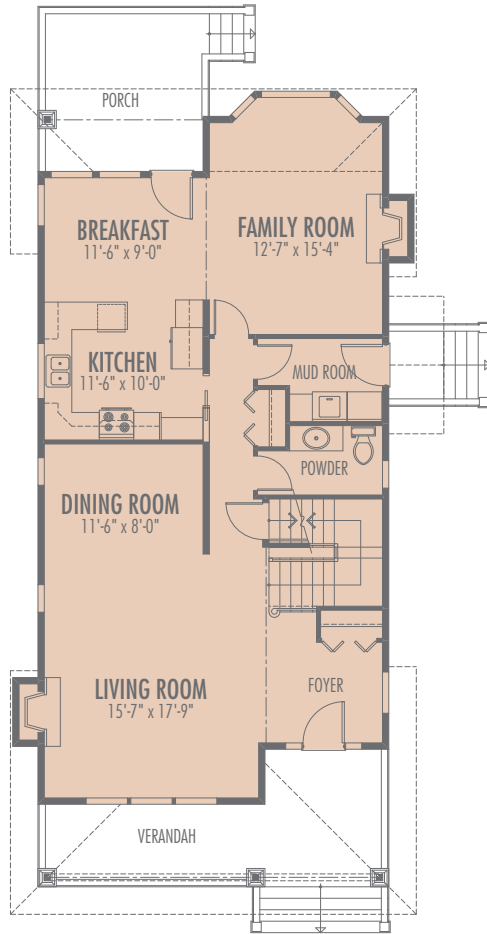
MAIN FLOOR
